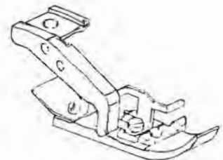
32747 32748 Presser Foot
