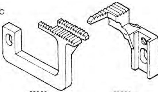
33828 Differential Feed Dog
