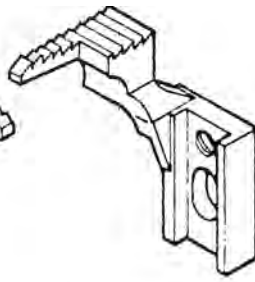
33829 Main Feed Dog
