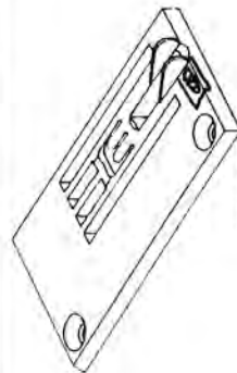
257090B64 Needle Plate
