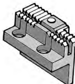
244756 Feed Dog. 11 Teeth, 16 Teeth to 1"
