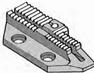
275005 (Medium Needle Hole) 275007 (Large Needle Hole) Feed Dog
