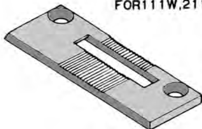
240144 Throat Plate
