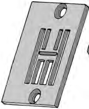
541938 Throat Plate
