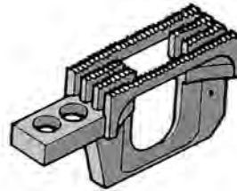
Feed Dog
