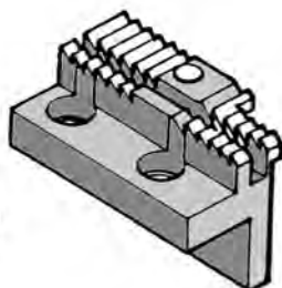
240075 Feed Dog
