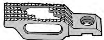
139499-501 Feed Dog, 12 Teeth, 8 Teeth to 1"
