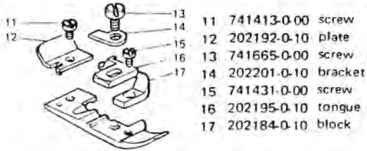
202171-3-10 presser foot
