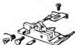
205034-3-12 (205034-3-11) Foot comp.
